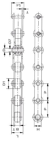
Double pitch roller chains straight plates with hollow pin
