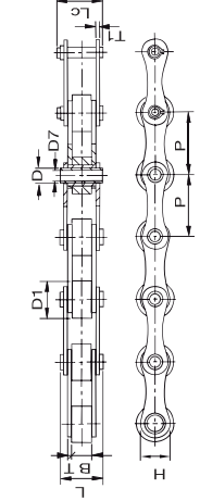
Type B Roller
