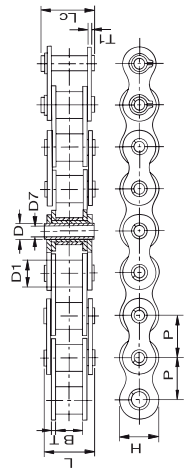
Type A fixed bush
